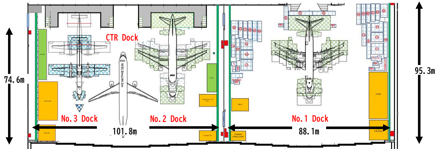
TOP VIEW
